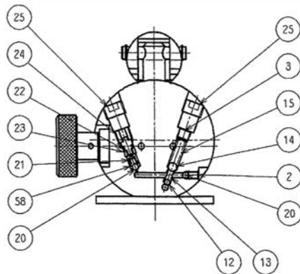
High pressure part cross section
